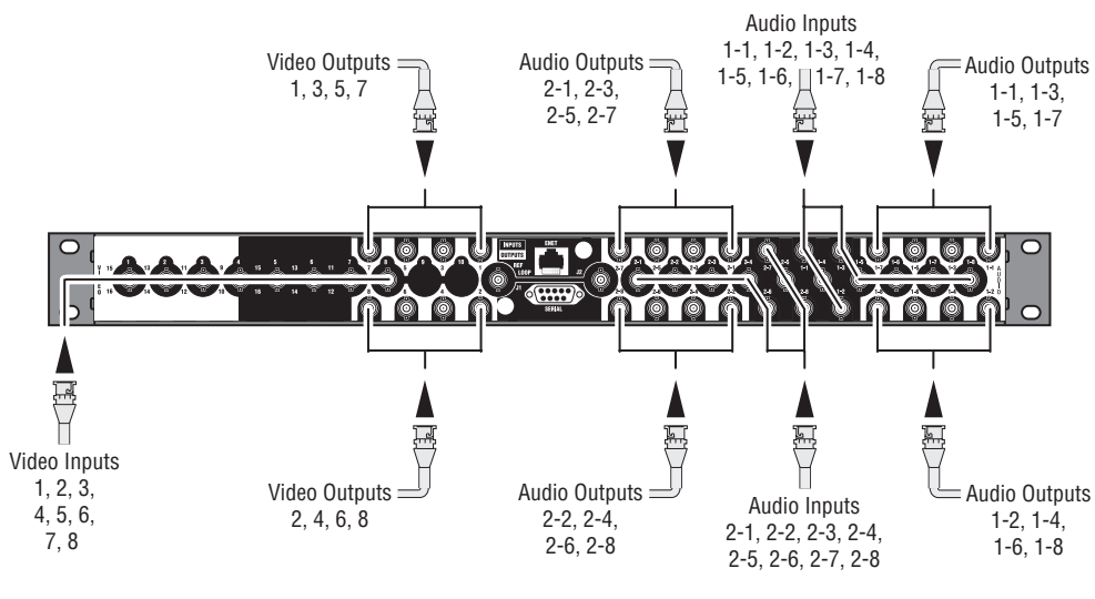
Cabling for Acappella Digital 16 x 16 Router
