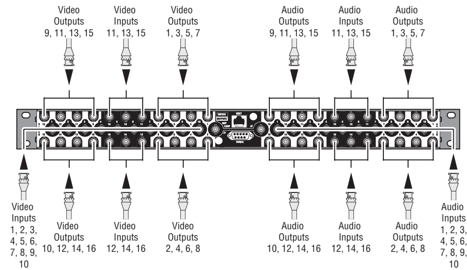
Cabling for Acappella Digital 16 x 16 Router
