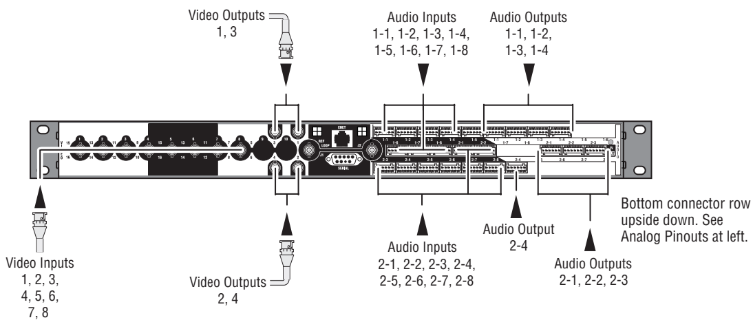
Cabling for Acappella Analog 16 x 16 Router
