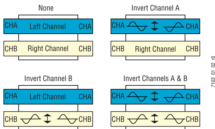
Figure 14. AES Inverts
