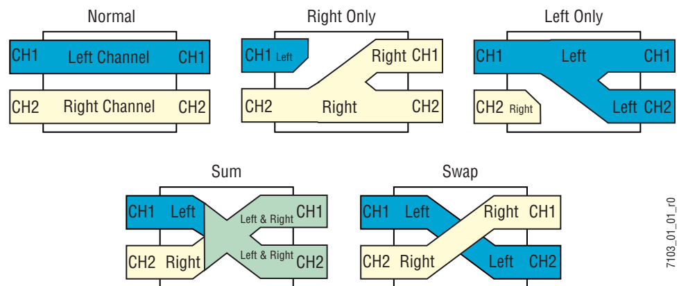
Figure 12. AES Attributes
