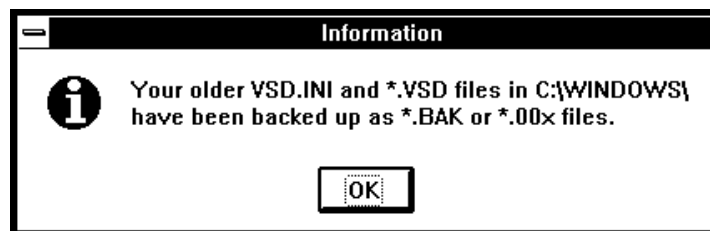
Figure 12. Information Window
