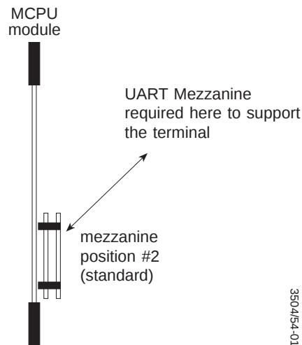
Figure 2. Amezi Mezzanine Location
