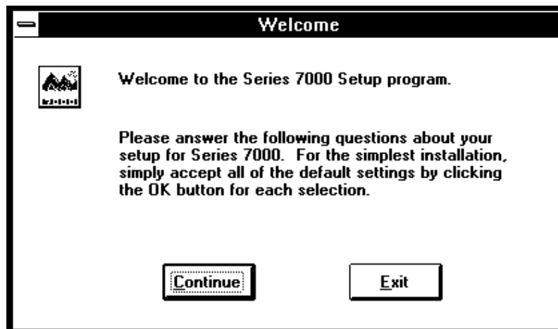
Figure 6. Welcome window
