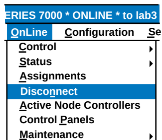
Figure 4. Disconnect Menu
