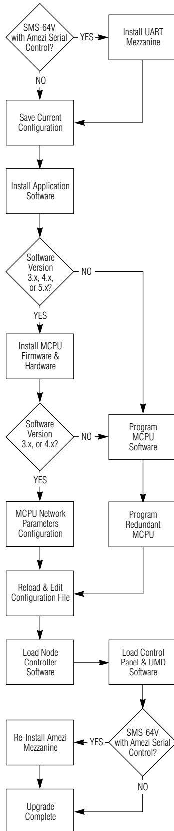
Figure 1. Upgrade Flowchart
