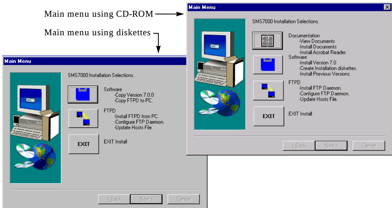
Figure 77. Main Menu
