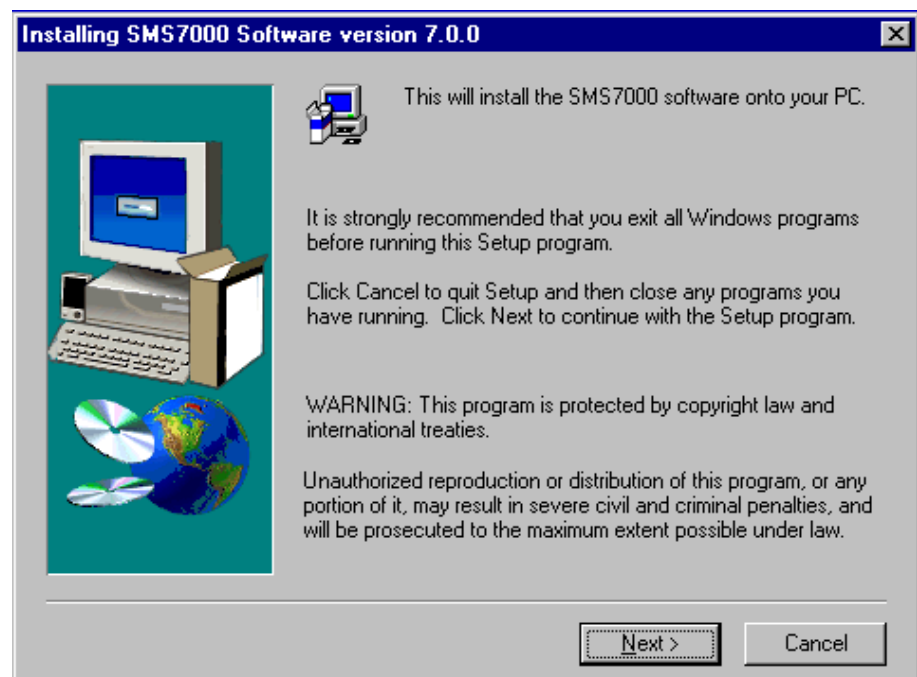
Figure 48. Information Window
