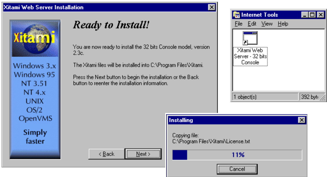
Figure 67. Install Windows
