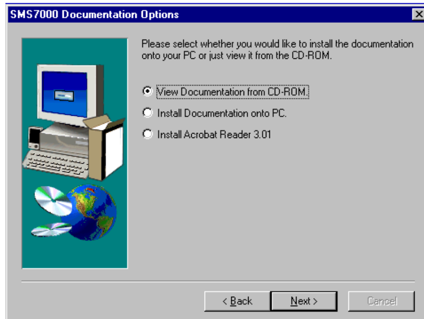
Figure 11. Documentation Window
