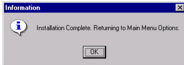
Figure 36. Information Window
