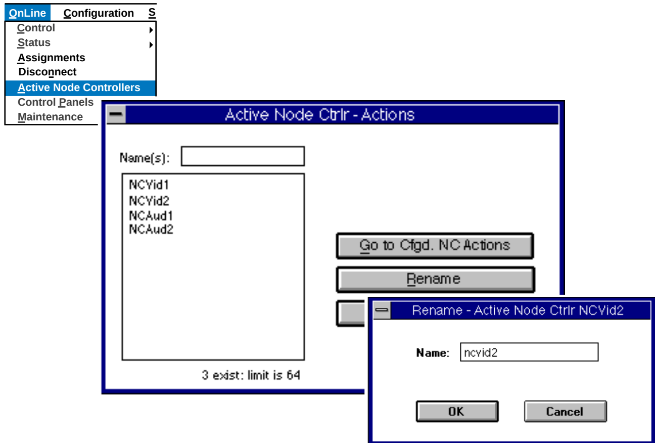
Figure 20. Active Node Controller Actions Window
