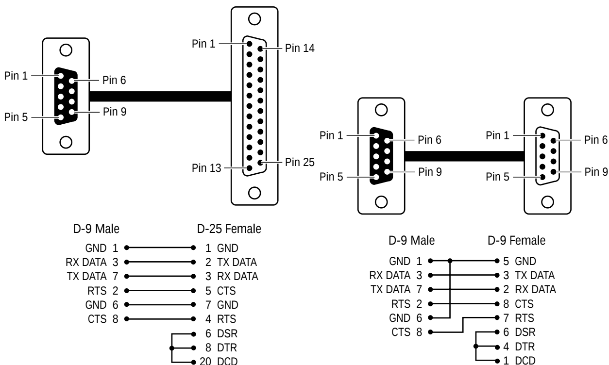
Figure 3. D Connector Pinouts
