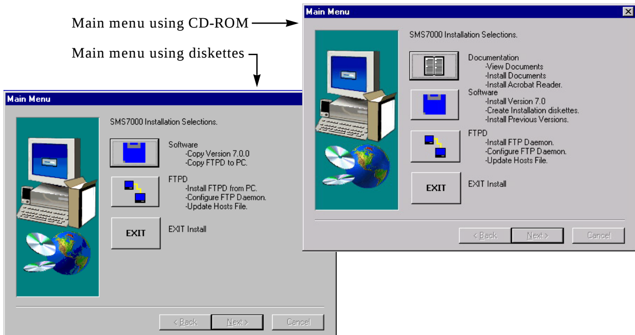
Figure 69. Main Menu
