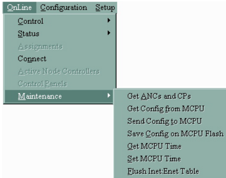
Figure 1. Maintenance Window
