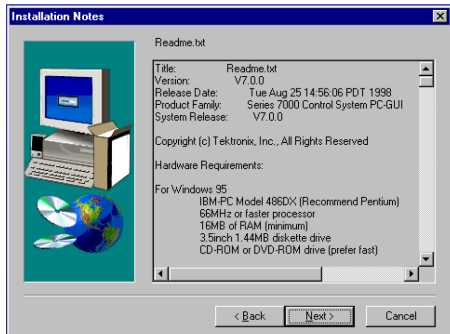
Figure 41. Readme.txt Window
