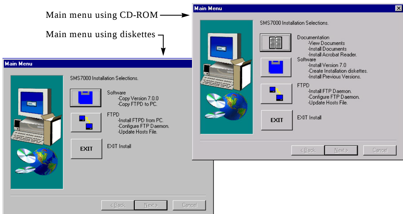
Figure 57. Main Menu
