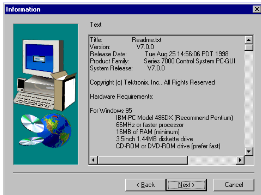
Figure 50. Information Window
